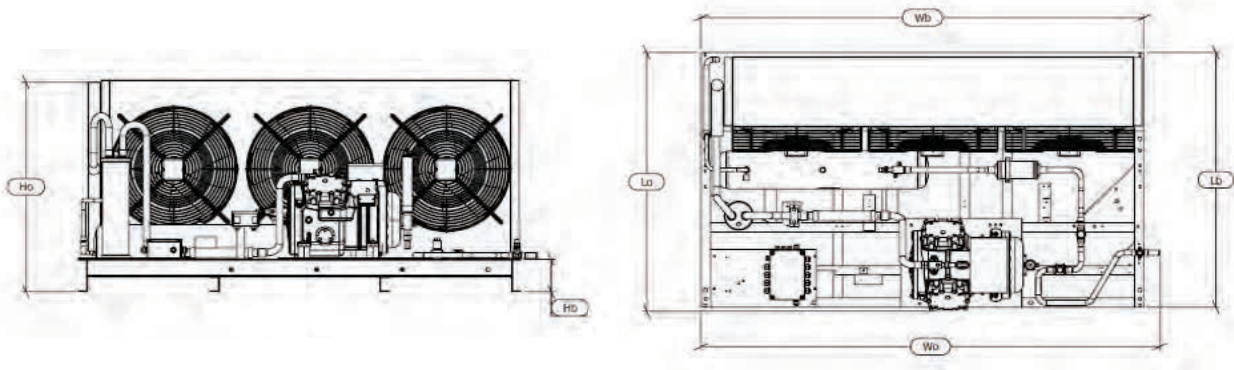
UNIT DIMENSION
