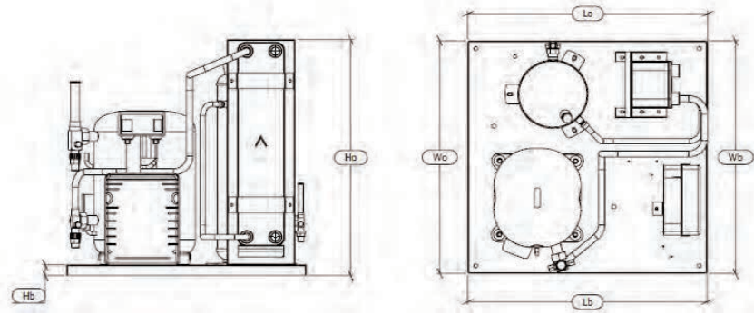
UNIT DIMENSION
